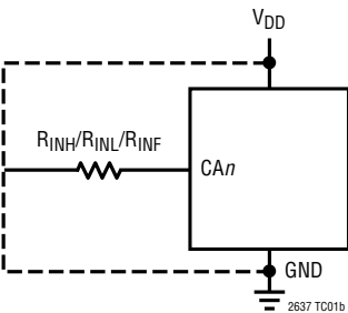
Test Circuit 2
